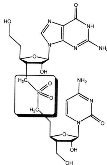
Figure 1. Structure of r(G_{SO_2}C) .
