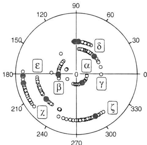
Figure 3. Backbone and glycosidic torsion angles of [r(\text{G}_{\text{SO}_2}\text{C})_2]_2 (●), compared with those of [r(\text{U}(\text{UA})_6\text{A})_2]_2 , 10 [r(\text{CGCGAAUUAAGCG})_2]_2 , 11 and [r(\text{CCCCGGGG})_2]_2 . 12 (○).
